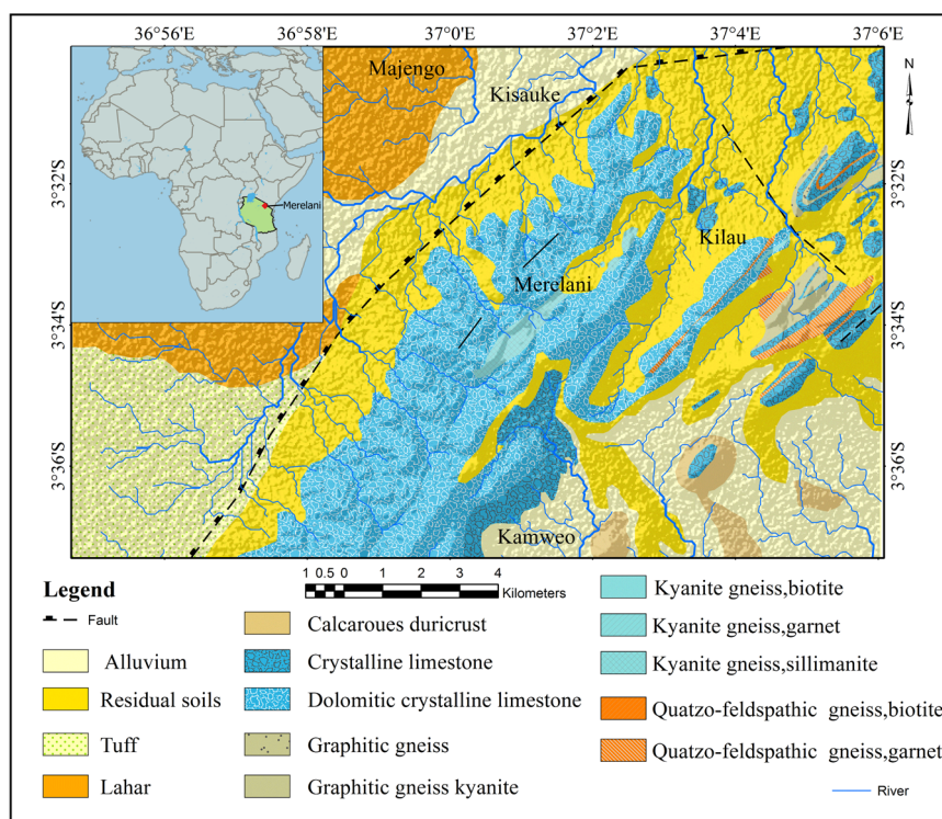
FIGURE 1. Mererani area location map (inset) and geological map indicating the lithological units around Mererani.
